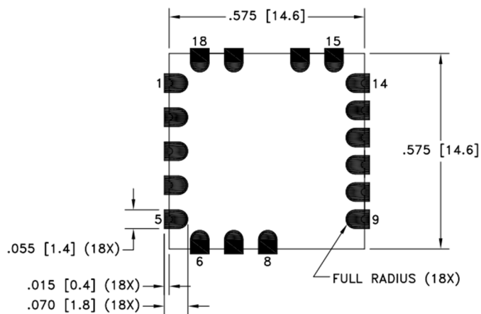
RECOMMENDED LAYOUT PATTERN TOP VIEW
